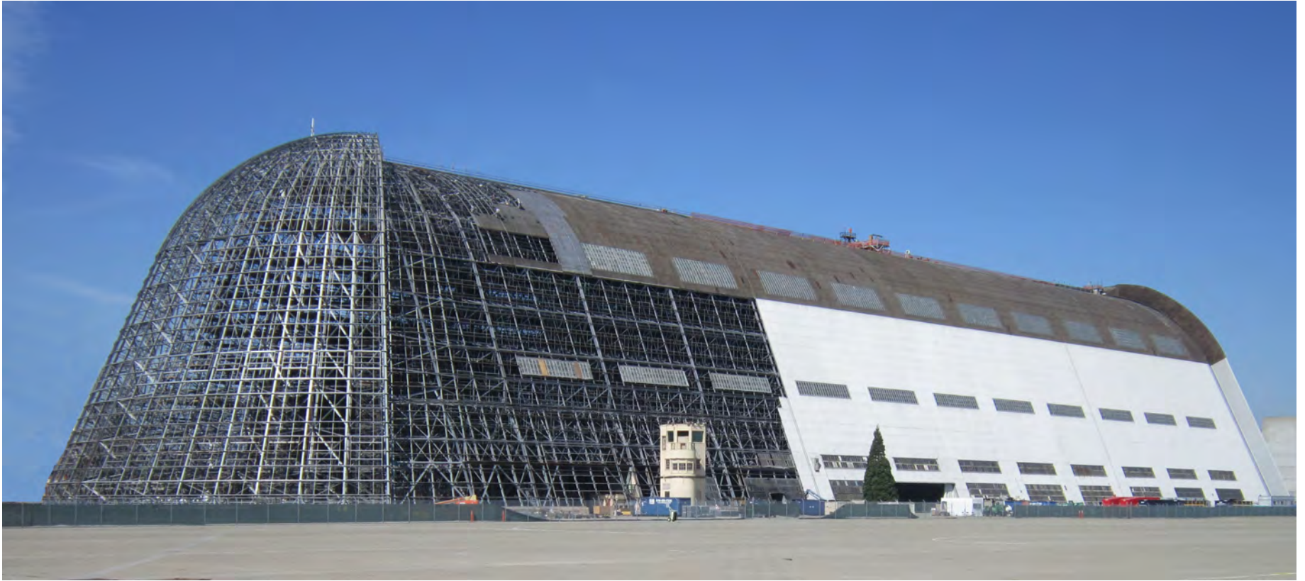
HANGAR 1 SIDE VIEW, BUILDING SKIN PARTIALLY REMOVED
