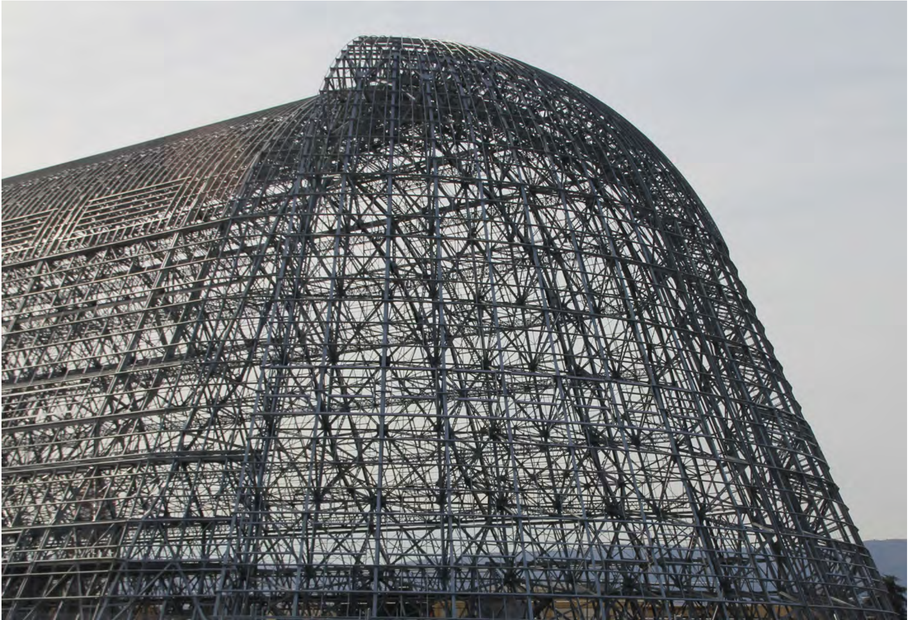
HANGAR 1 END VIEW, BUILDING SKIN REMOVED
