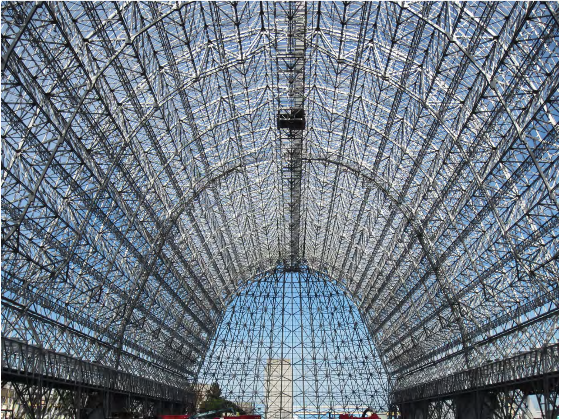
HANGAR 1 INTERIOR, BUILDING SKIN REMOVED
