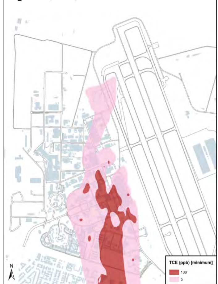
TCE concentration in the groundwater aquifer due to contamination from Regional (MEW) sources.
